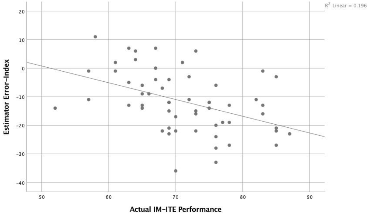
Scatterplot for actual IM-ITE and estimator error-index
